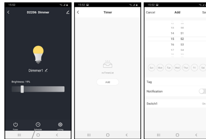
Pulsante "Schedule"
